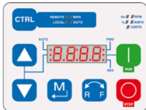
Keypad (11-45 kW)
